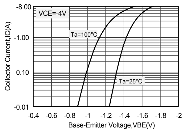
Fig6.Base-Emitter Voltage Characteristics
