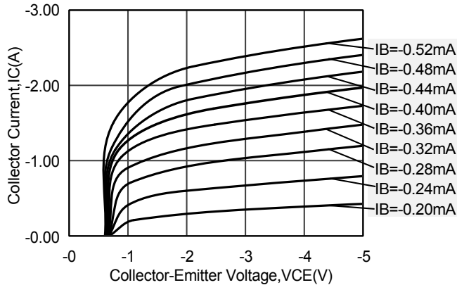
Fig1.Static Characteristics
