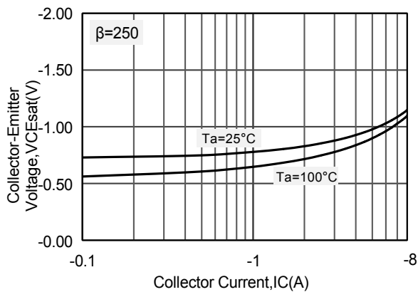
Fig3.Collector-Emitter Saturation Voltage Characteristics
