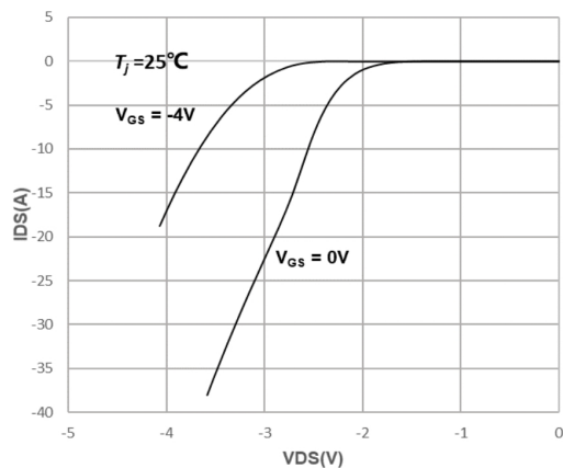
Fig9. Body Diode Characteristics
