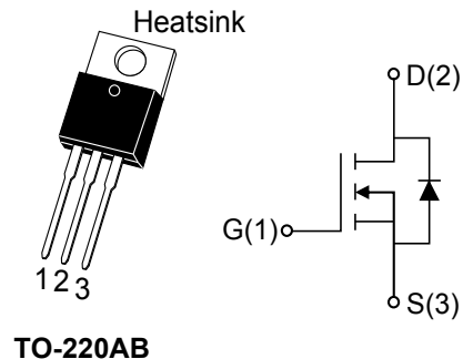
TO-220AB
