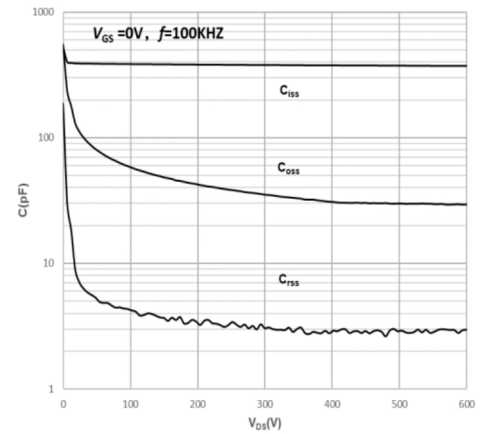
Fig8. Capacitances vs. Drain-Source Voltage (0-600V)
