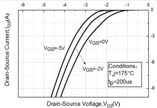
Fig10. Body Diode Characteristic at 175^\circ\text{C}
