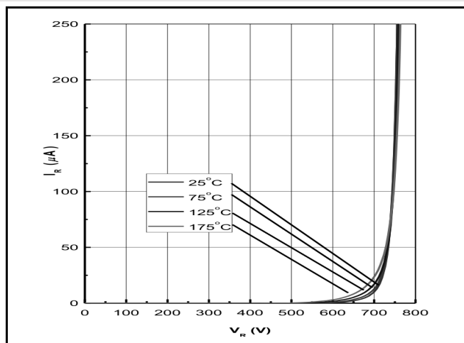
Figure 2 Reverse Characteristics
