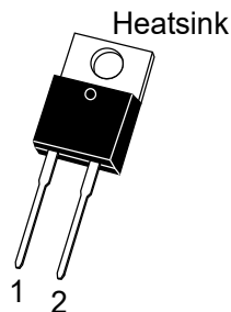
Package: TO-220AC-A SF802A SF802A-HF HF=Halogen Free
