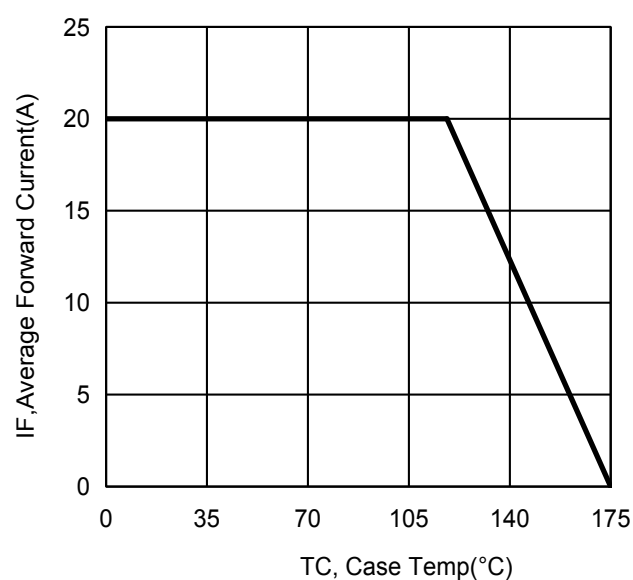
Fig2. Typical Current Derating Curve, Porelement
