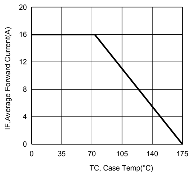
Fig2. Typical Current Derating Curve, Pavelement
