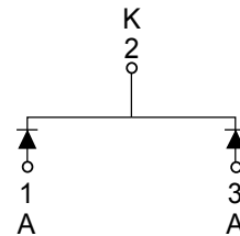
Package:TO-263M-2L MBR20H300M MBR20H300M-HF HF=Halogen Free
