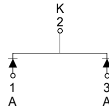
Package:TO-263M-2L EBR20L120M EBR20L120M-HF HF=Halogen Free
